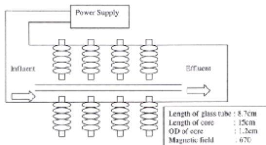
Fig. 2. Schematic Diagram of general magnetic reactor (electromagnets) for sewage treatment 37
